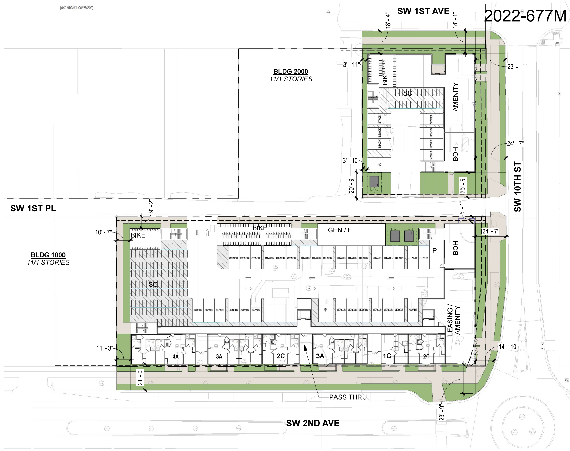
1 SITE PLAN 1" = 40'-0" 0' 20' 40' 80'
