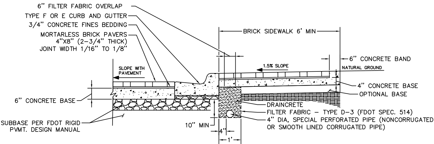
BRICK ROADWAY SECTION
