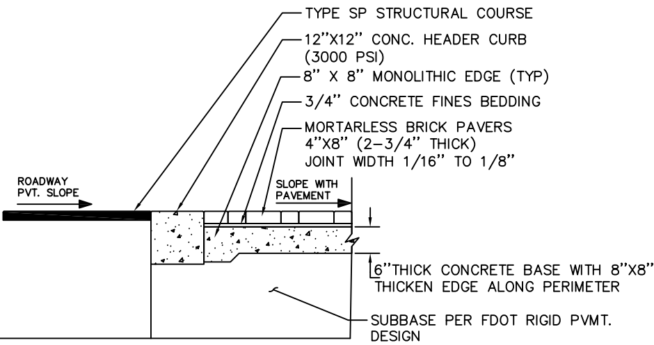
CROSSWALK SECTION
