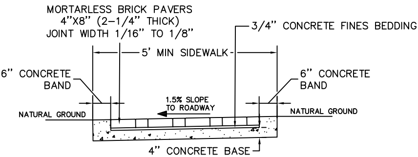
BRICK & SIDEWALK SECTION NOT ADJACENT TO CURBING
